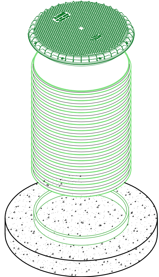
ISOMETRIC
