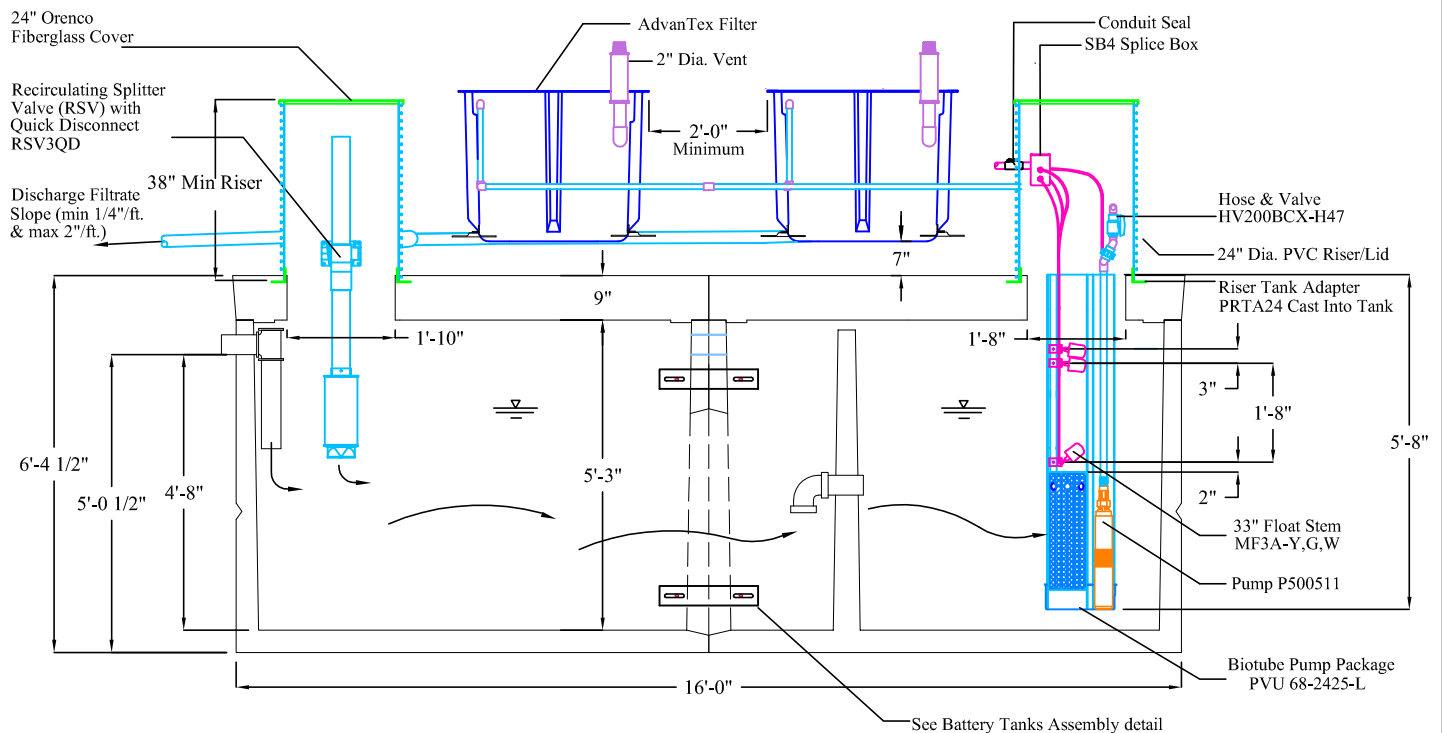
ELEVATION VIEW
