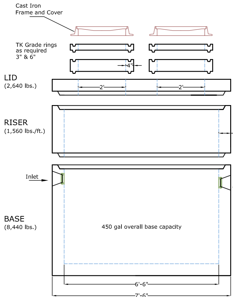
FRONT ELEVATION
